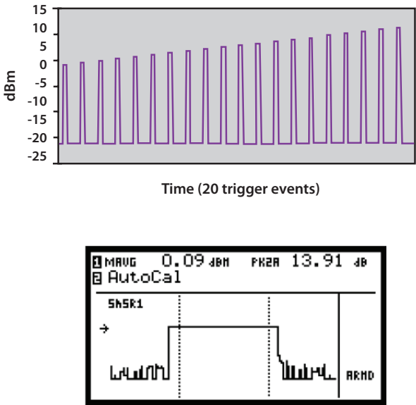
Figure 8.2.2. Power Sweep and power meter measurement of a single pulse within the sweep
