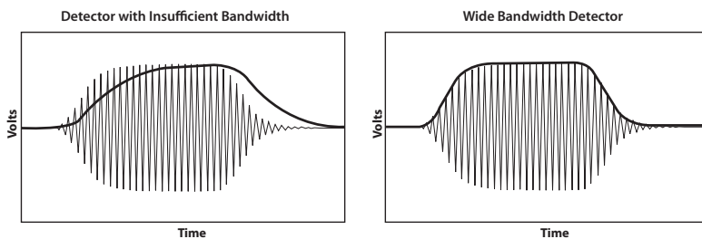
Figure 2.2.3. A Wide Bandwidth Detector Correctly Tracks a Pulse Envelope
