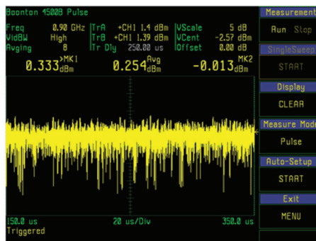
Figure 8.3.6. A noise-like CDMA communication signal displayed in the time domain
