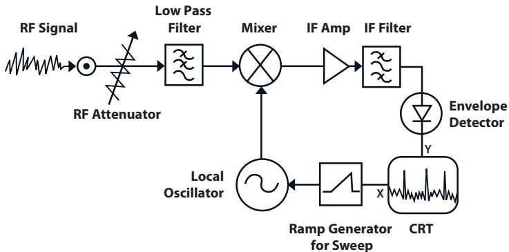
Figure 4.4.2. Typical front-end of a Superheterodyne Spectrum Analyzer
