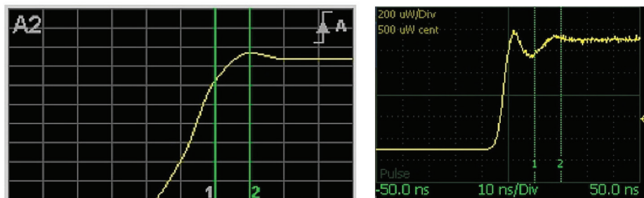
Figure 6.2.5. Screen shot of under-sampled rising edge on left and well-defined, over-sampled edge on right
