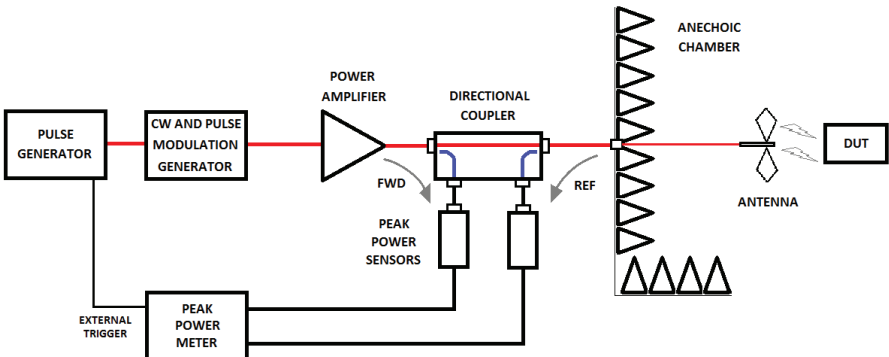
Figure 7.3.4. Accurate Monitoring of delivered power
