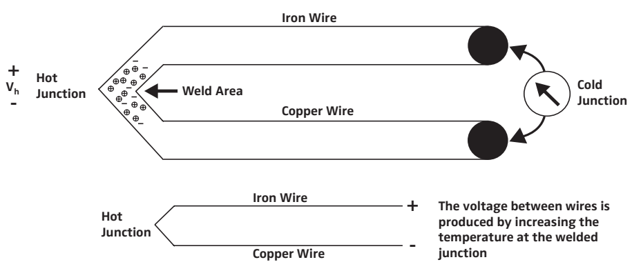
Diagram illustrating Thermocouple Principle
