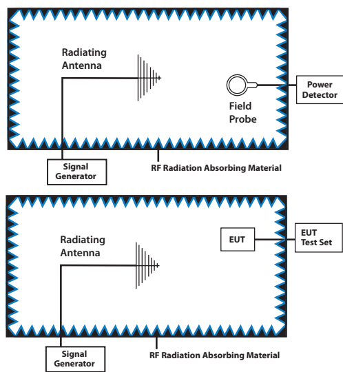
Figure 7.3.3. The Substitution Method Diagram
