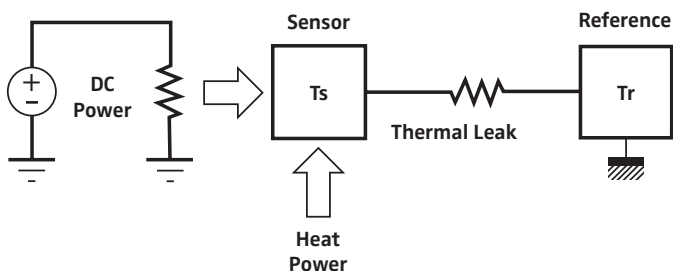
Bolometer Diagram
