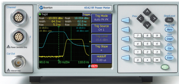
Boonton 4542 RF Power Meter
