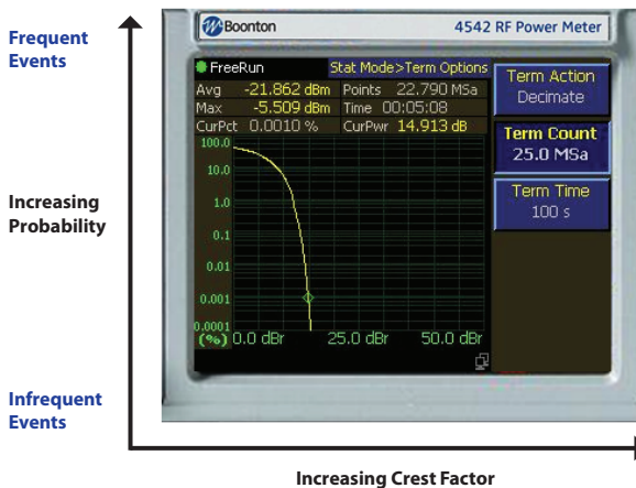
Figure 8.3.5 CCDF of a modulated communication signal
