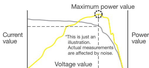
Typical voltage, current, and power measurements in MPPT control
