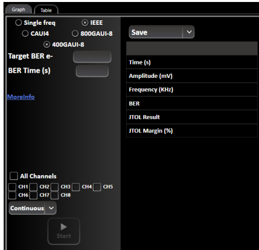
Figure 6: Automated IEEE JTOL
