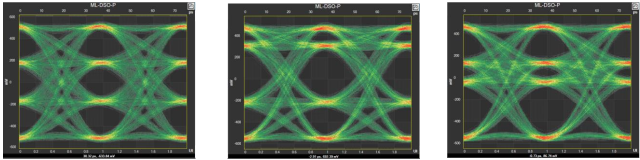
Figure 16: Inner/Outer Eye Control Using ML4079EN
