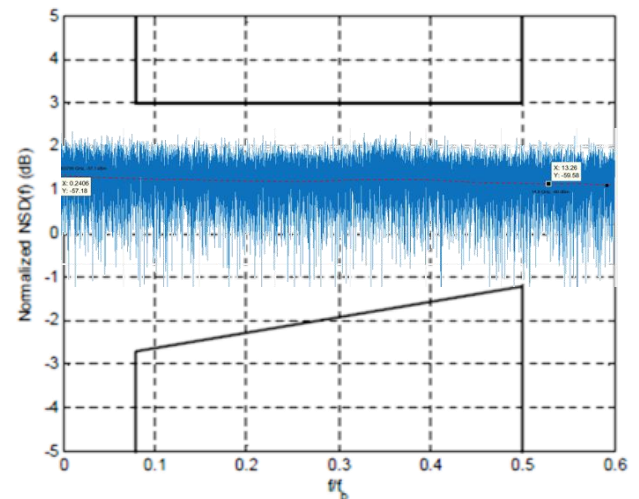
Figure 11: Noise Flatness
