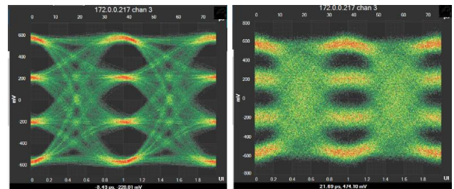
Figure 14: Eye Diagram before and after noise injection – PAM4 modulation
