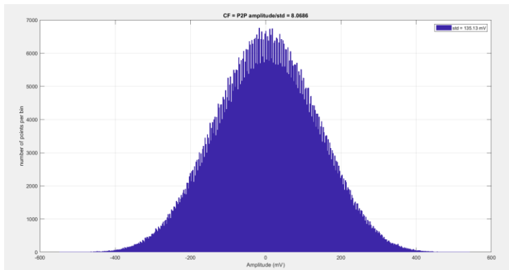
Figure 10: Crest Factor Measurement: Gaussian Noise
